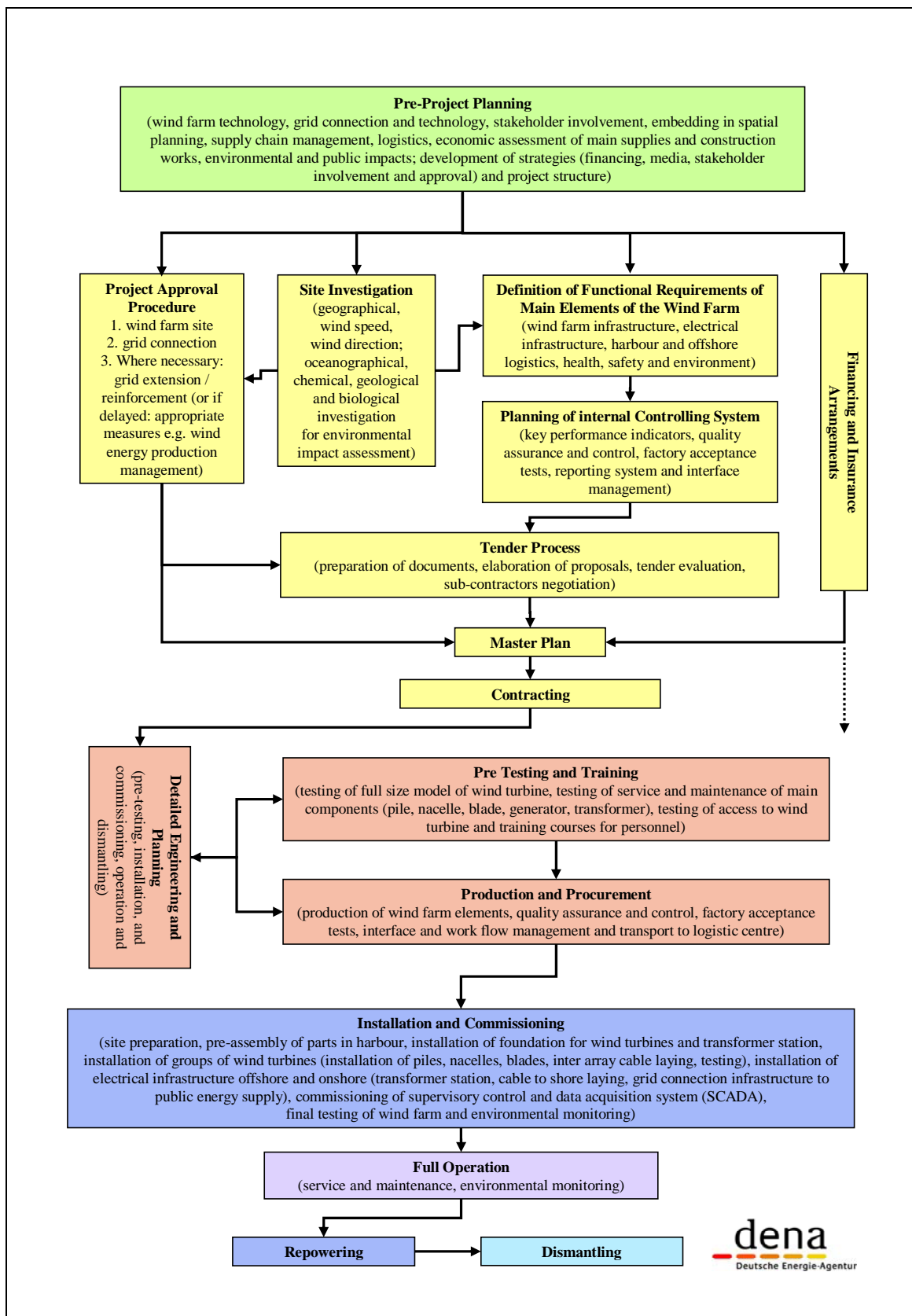
Figure 2: Flow chart of the main work packages for the phases of offshore wind farm planning and realisation.
